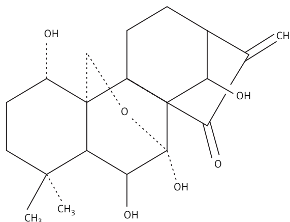
Fig. 1. Chemical structure of oridonin
