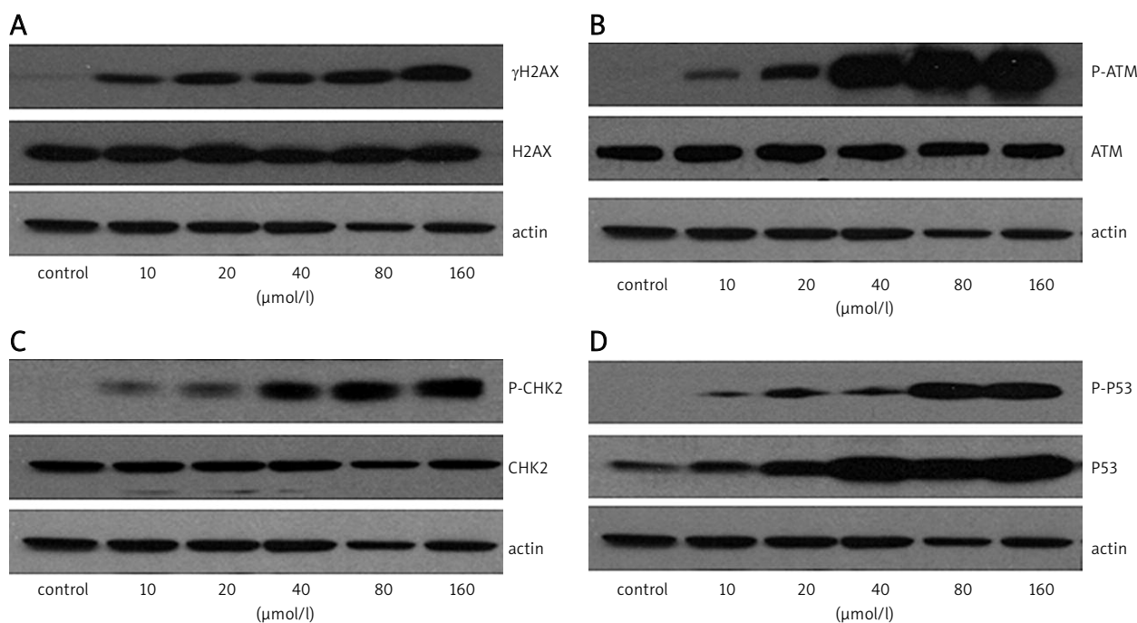
Fig. 5. Western blotting analysis of expression of \gamma H2AX (A), P-ATM (B), P-CHK2 (C), and P-P53 (D) protein. The MCF-7 cells were treated with different concentrations of oridonin. Total cellular proteins were harvested and subjected to Western blotting analysis. \beta -actin was used as a loading control
