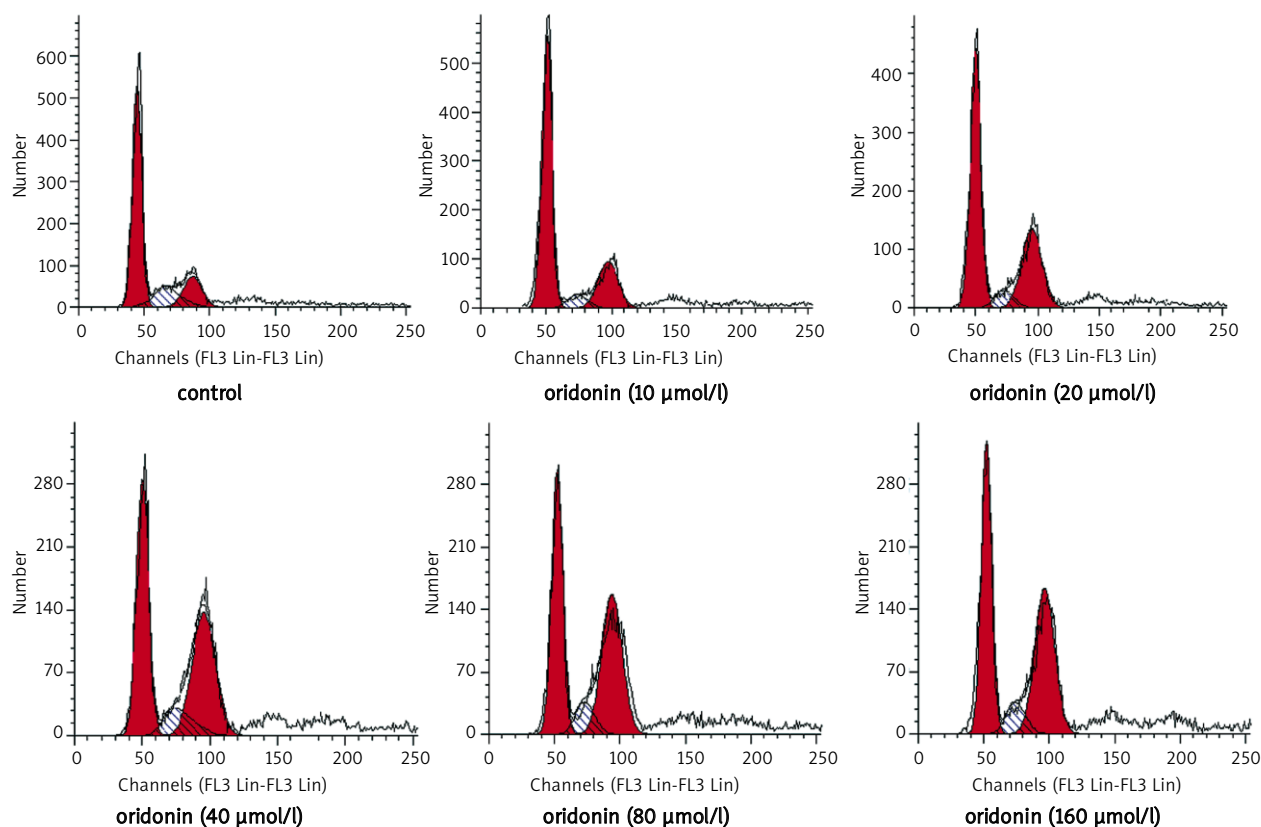
Fig. 3. Effects of oridonin on cell cycle distribution in cultured MCF-7 cells. Flow cytometric analysis of the DNA content in control and oridonin-treated groups (10, 20, 40, 80 and 160 µmol/l) for 48 h
