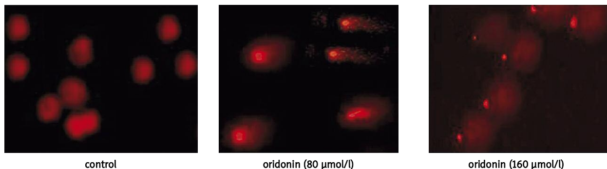
Fig. 2. Effect of oridonin on DNA damage. DNA damage as detected using an alkaline comet assay 48 h after oridonin treatment in MCF-7 cells. Photomicrographs of damaged DNA after the various oridonin treatments showing an increase in the tail length and tail moment
