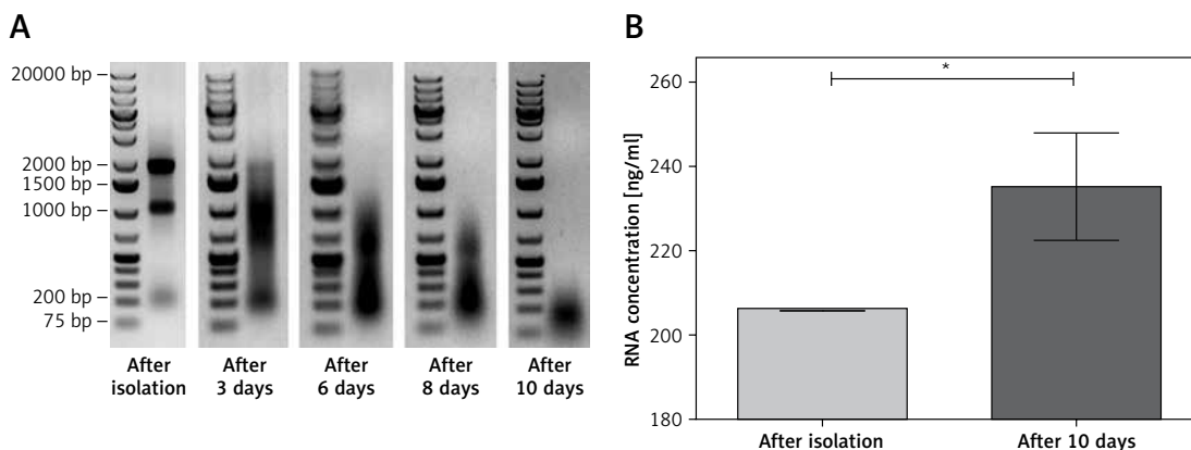
Figure 3. Degradation of RNA used for cDNA synthesis. A – Native electrophoresis in 1% agarose gel of RNA samples at different time points. Marker GeneRuler 1kb Plus DNA Ladder (Thermo Scientific). B – Mean RNA concentration measured immediately after isolation and after 10 days of incubation at room temperature
