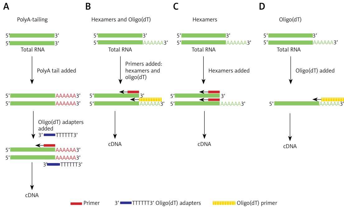
Figure 1. Comparison of different reverse transcription kits used to quantify lncRNA employing qRT-PCR methods. A – cDNA synthesis using random hexamer primers preceded by polyA-tailing and adaptor-anchoring steps, B – simple reaction using blend of random hexamer primers and oligo(dT), C – reaction based on random hexamer primers, D – based only on oligo(dT)
