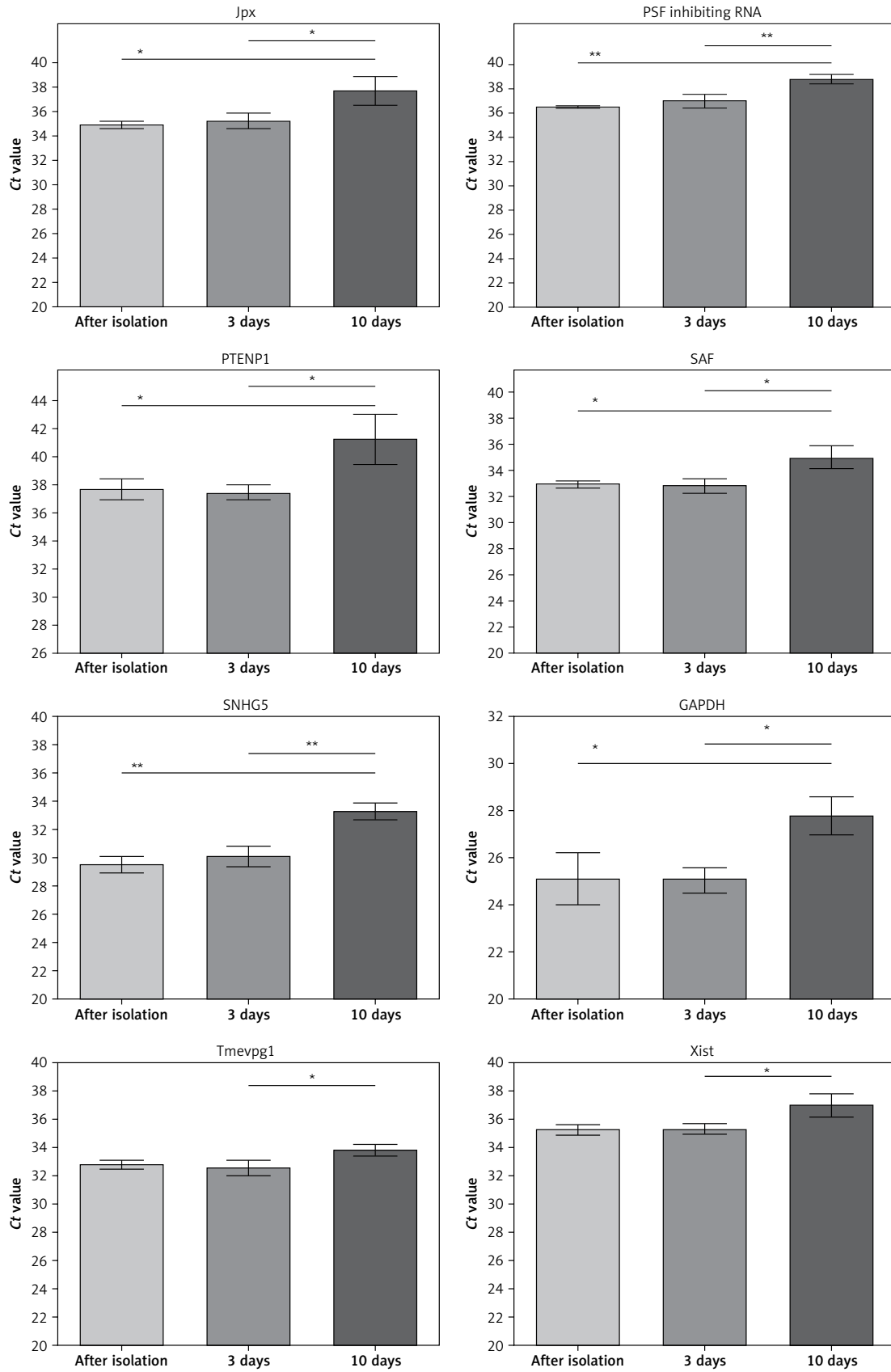
Figure 4. Comparison of mean Ct values of changed lncRNAs and GAPDH mRNA amplified with cDNA synthesis using random hexamer primers preceded by polyA-tailing and adaptor-anchoring steps and RNA samples just after isolation and after 3 and 10 days incubation at room temperature
